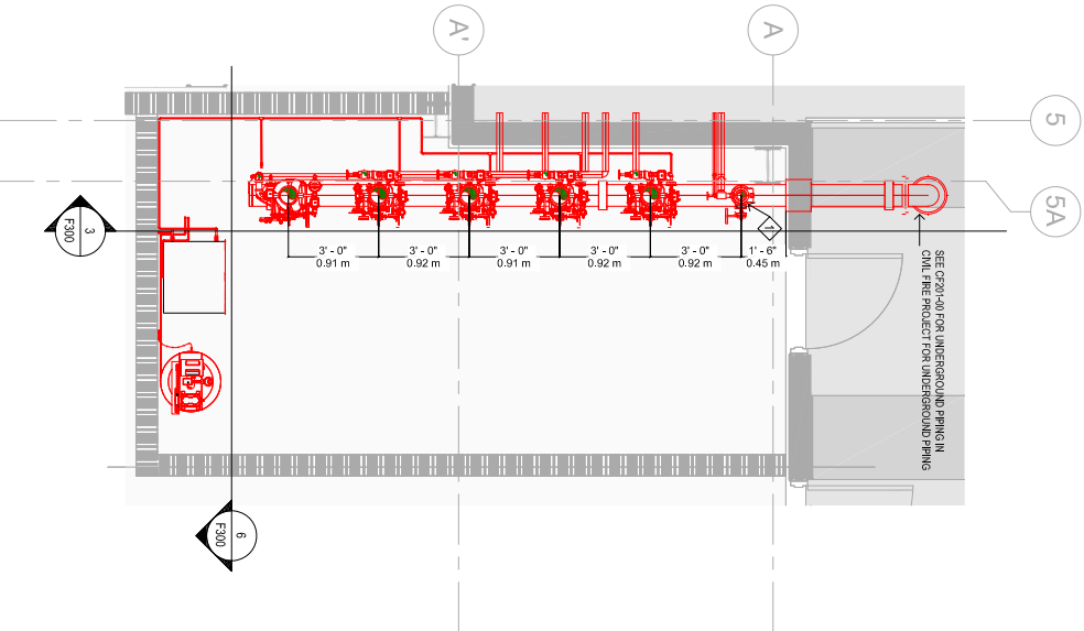
1 FIRE PROTECTION BUILDING 01 - RISERS ROOM PLAN VIEW
